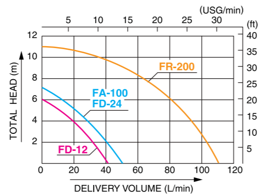
■ Performance Curve
